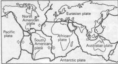
Left: The Earths Plates
